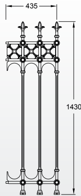
Stirling half height railing panel (33kg)
