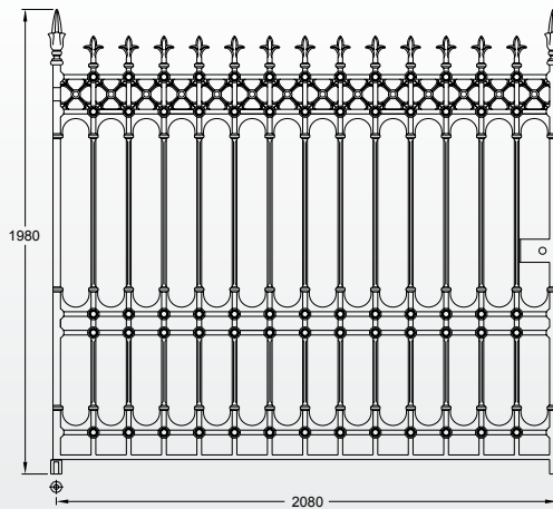
Stirling driveway gate (14 x 6.5ft pair, 620kg)
